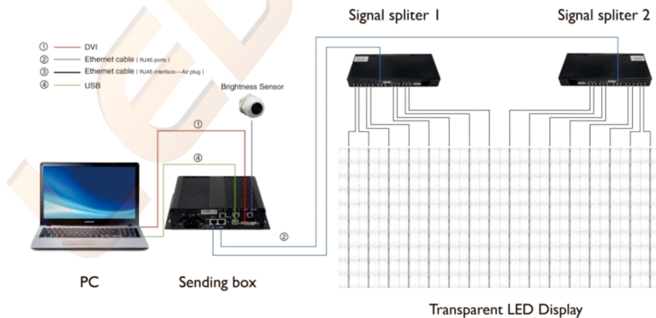
Topological diagram of the TW transparent LED screen
